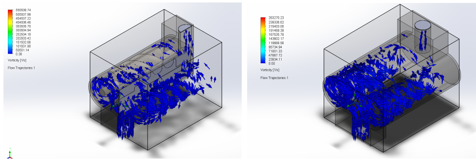
Figure 2. Particle trajectories and flow velocity distribution in the working chamber of a three-screw compressor.
