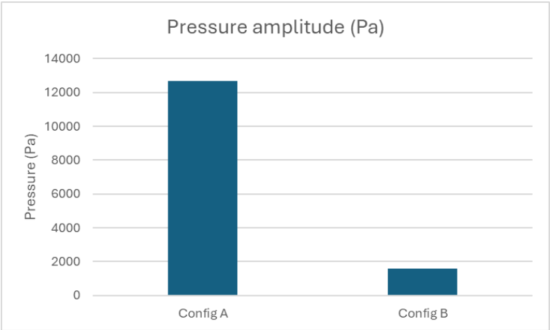
Figure 5. Amplitude of static pressure fluctuations.
